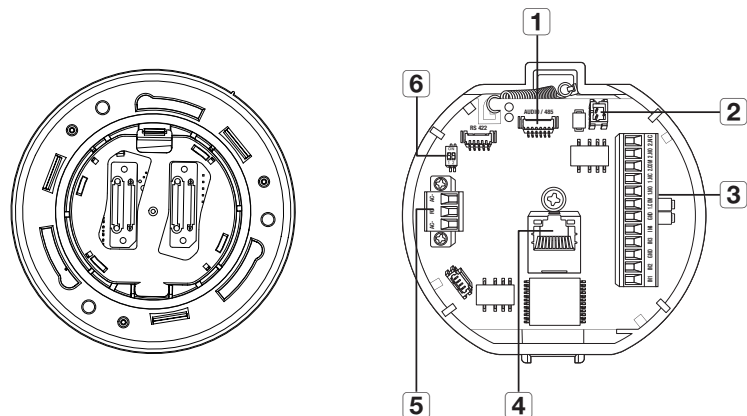
Bottom View of Installation Base
