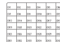
36-split mode
