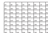
64-split mode
