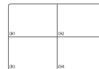
4-split mode
