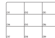
9-split mode
