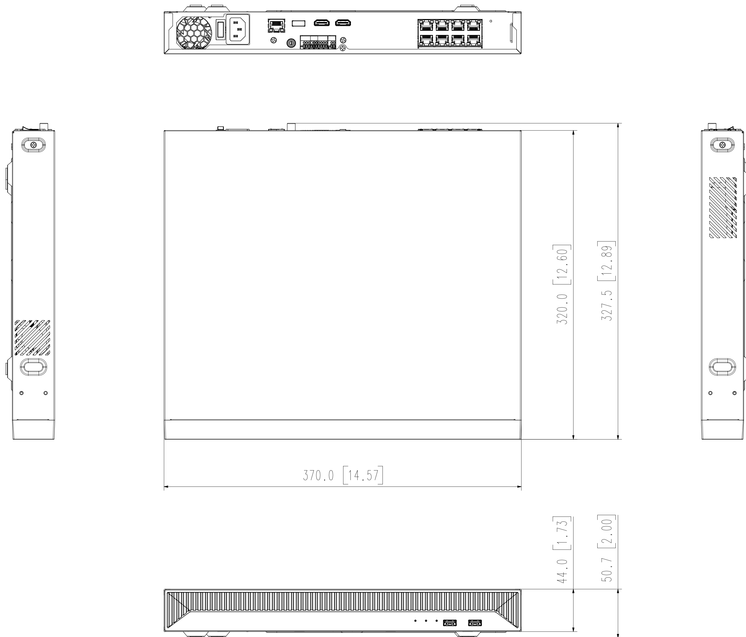
Appearance Drawing XRN-815S Unit : mm[inches]
